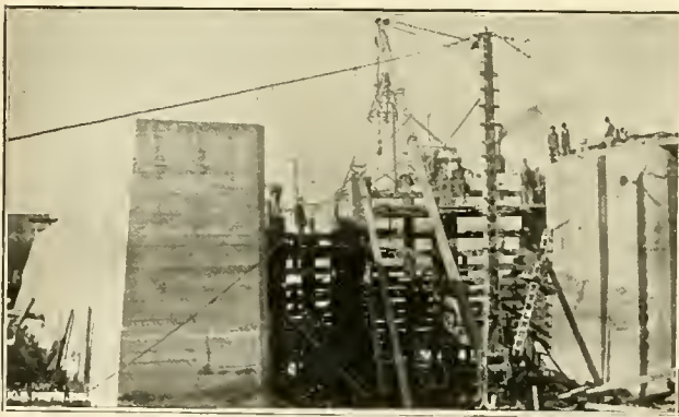
Building of Lock Gate on Upper Side.
